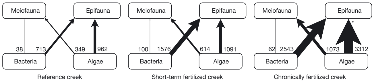
Fig. 6. Fluxes between benthic bacteria and algae and their meiofaunal and epifaunal grazers ( \mu\text{g C m}^{-2} \text{d}^{-1} ) in the 3 creeks studied. An asterisk indicates significant ( p < 0.01 ) differences in flux (ANOVA; Tukey test)
